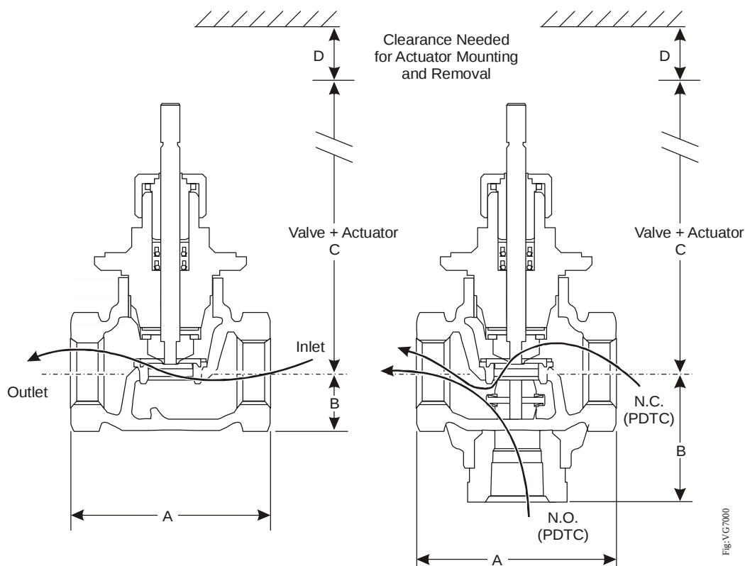
Figure 2: Two-Way Normally Open (N.O.)/Push Down to Close (PDTC), Two-Way Normally Closed (N.C.)/Push Down to Open (PDTO), and Three-Way Mixing Valve Dimensions, Fluid Flow Directions, and Port Designations (Refer to Table 1 and Table 2.)
