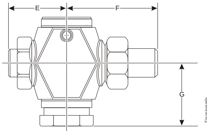
Figure 4: Two-Way N.O./PDTC Union Angle Valve Dimensions (Refer to Table 4.)
